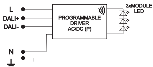
1. Light source LED (basic version - programmable driver)
