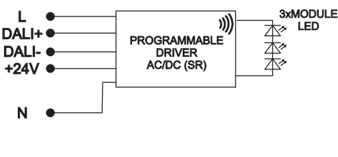
3. Light source LED (II Class) (version as an option - Sensor Ready driver)
