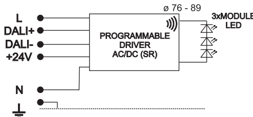
2. Light source LED (I Class) (version as an option - Sensor Ready driver)
